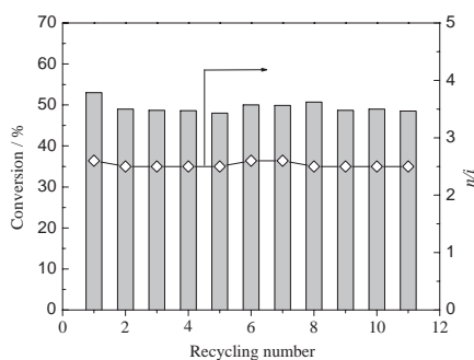
Figure 1. The recycling results of 1-hexene hydroformylation over catalysts TMGL–TPPTS–Rh/MCM-41. TMGL loading = 10 wt %, Rh loading = 0.8 wt % based on silicas, TPPTS/Rh = 5 (molar ratio).
